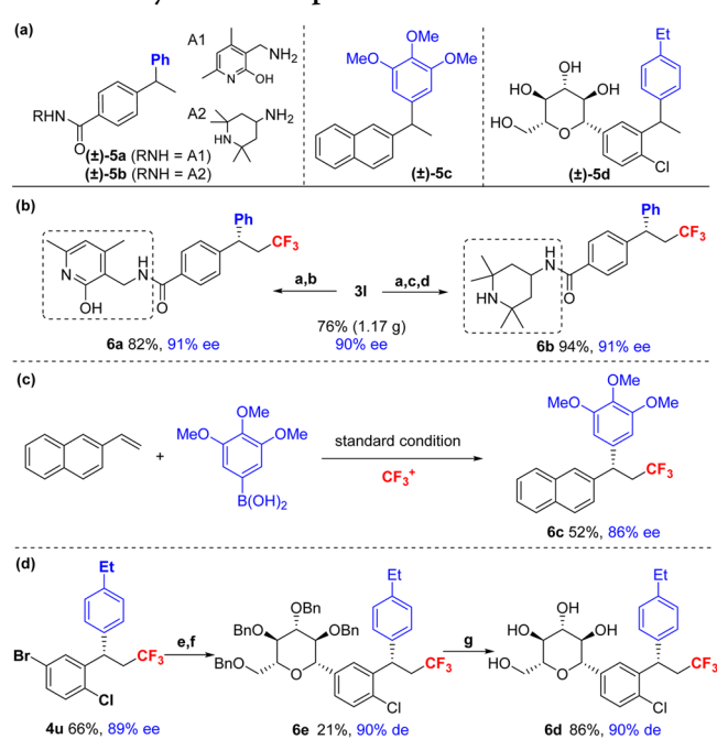
Scheme 2. Synthesis Compounds a
