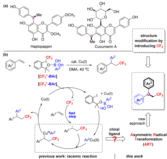
Scheme 1. Proposed ART Reaction for the Synthesis of Chiral CF 3 -Substituted 1,1-Diaryllalkanes
